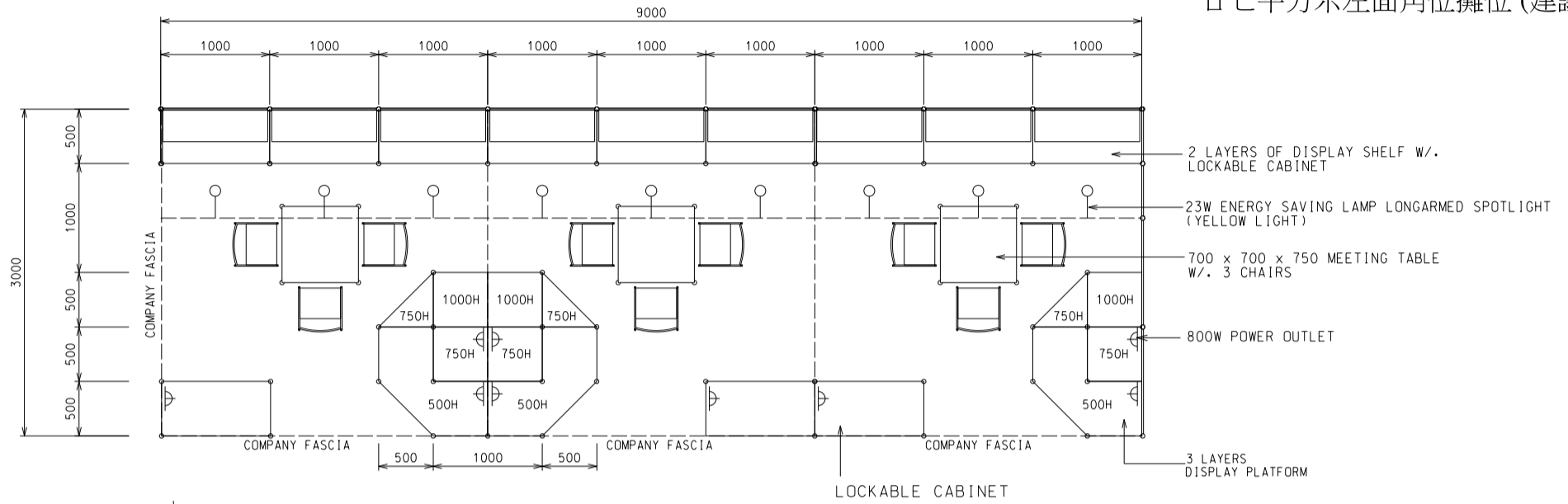
PLAN 9M(W) X 3M(D) X 2.5M(H) LEFT CORNER BOOTH B
